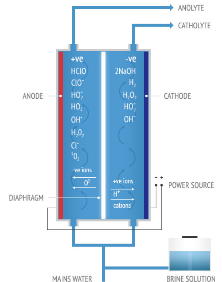
Drawing of Envirolite operational principle
